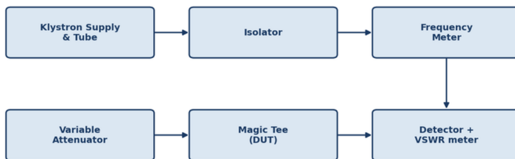
Fig. 1 — Microwave bench setup with magic tee as device under test
